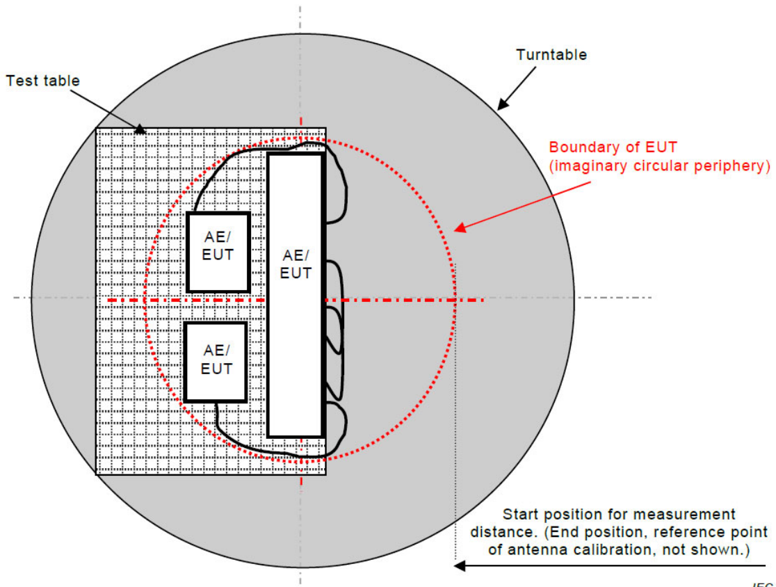
Figure C.1 – Measurement distance
