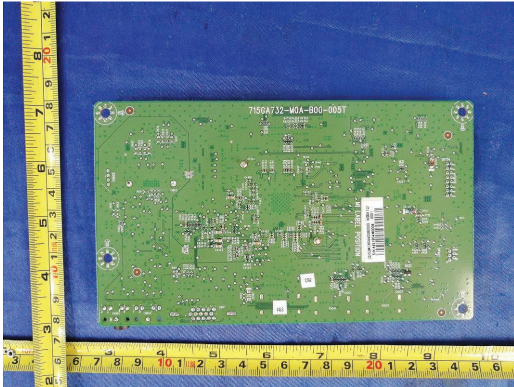
Figure 13. Main board 715GA732
