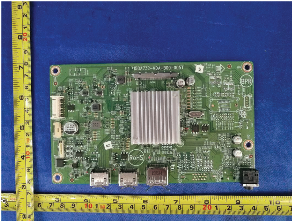
Figure 12. Main board 715GA732
