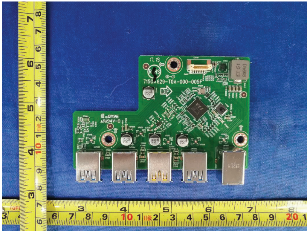
Figure 14. Extend USB board 715GA629
