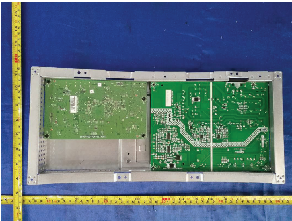
Figure 8. Internal view
