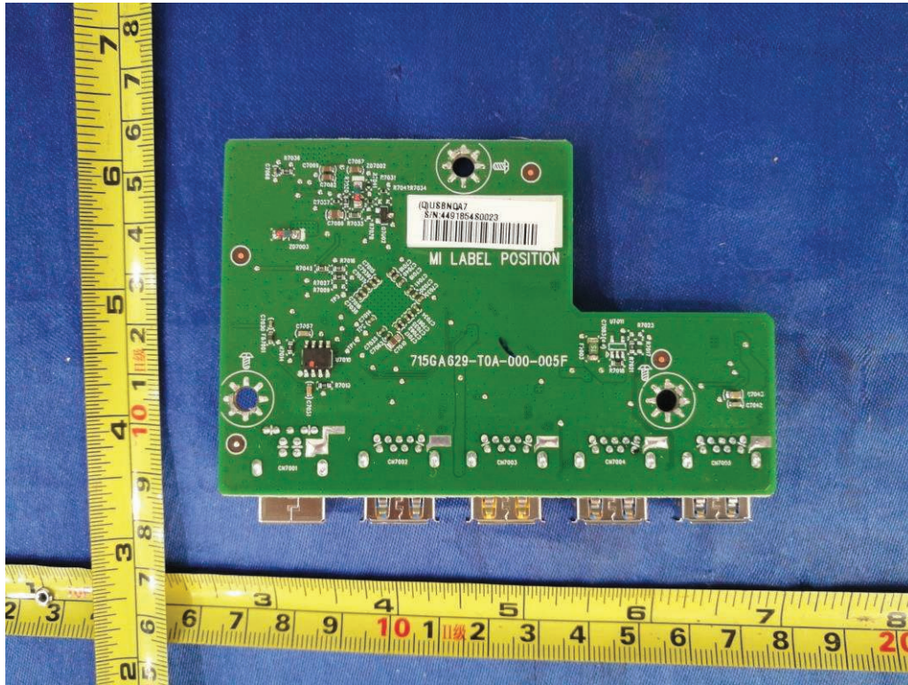
Figure 15. Extend USB board 715GA629
