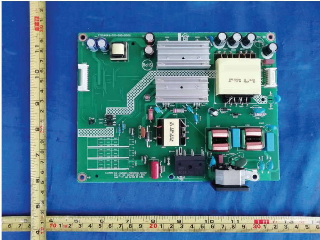
Figure 10. Power board 715GA649
