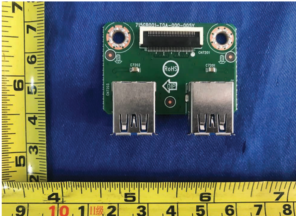
Figure 59. USB board 715GB001
