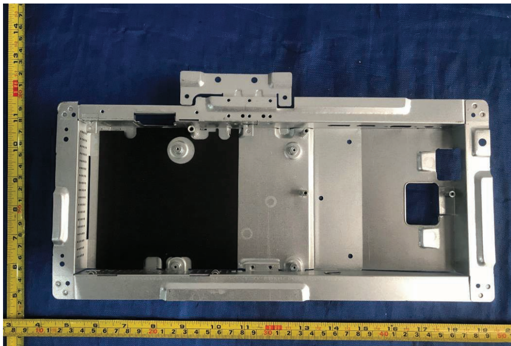
Figure 34. Internal view of metal enclosure
