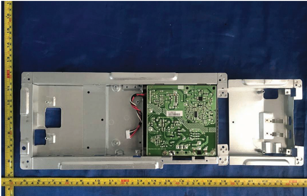
Figure 11. Internal view of metal enclosure
