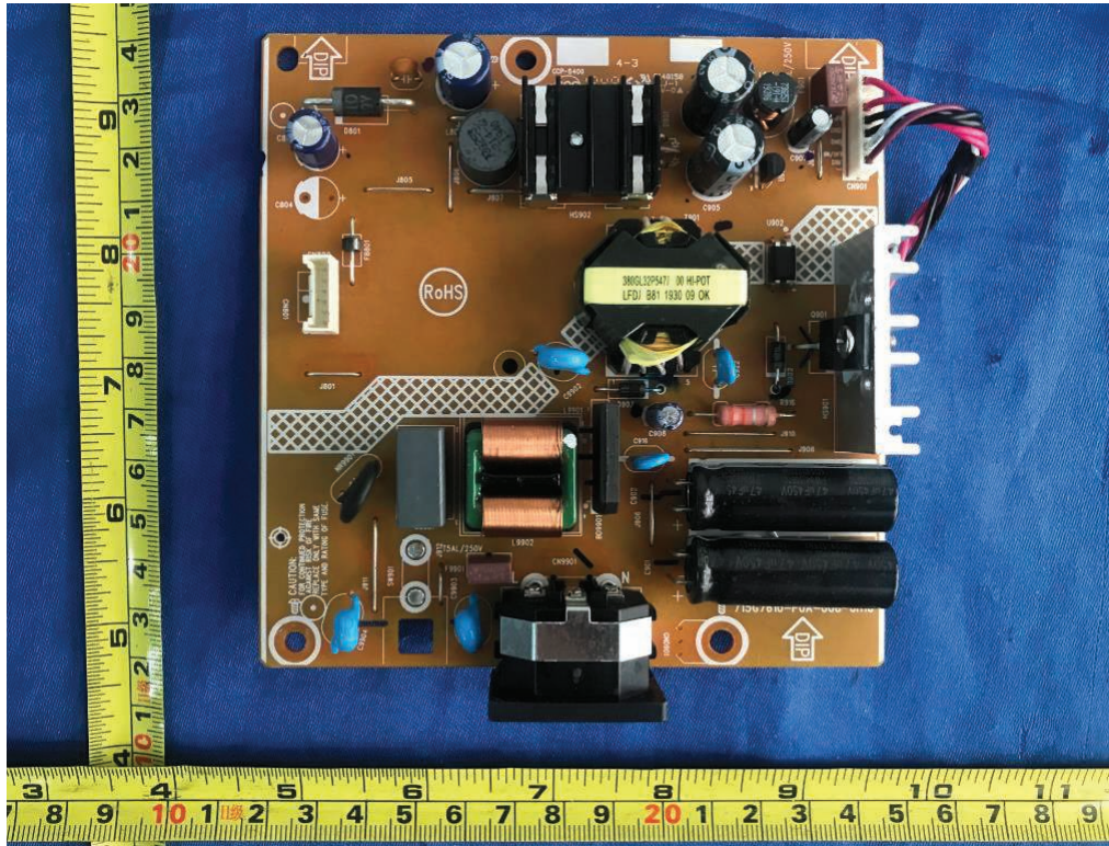
Figure 35. Power board 715G7610 (without AC switch)
