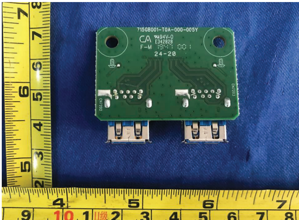
Figure 60. USB board 715GB001
