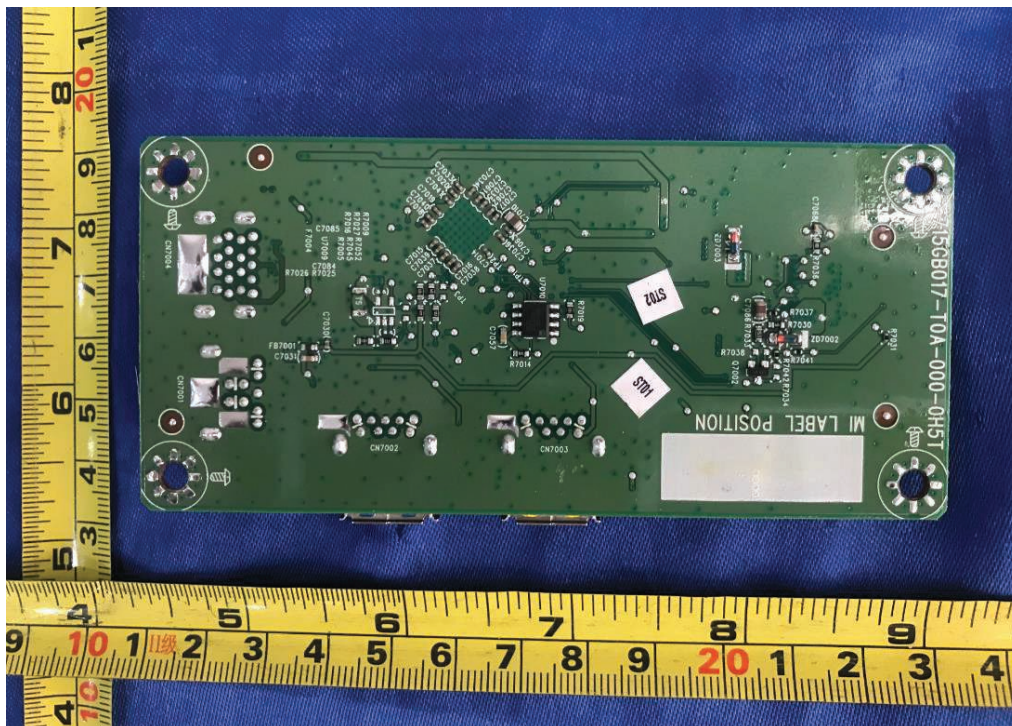
Figure 24. USB board 715GB017
