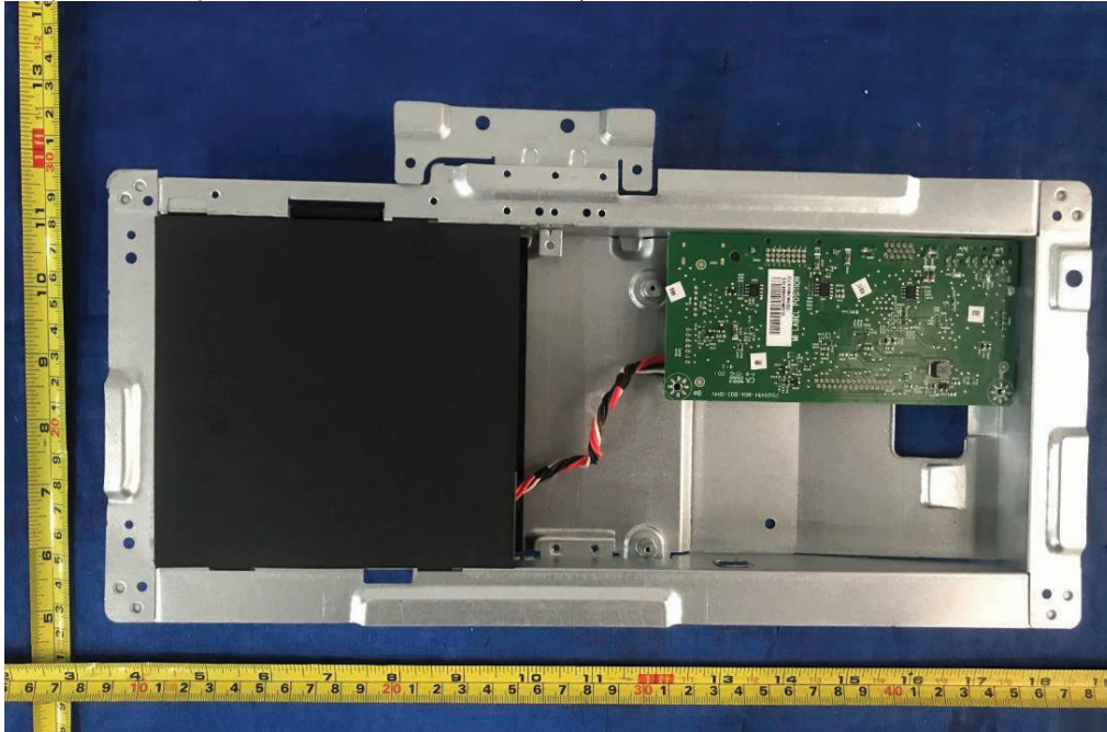
Figure 37. Internal view of metal enclosure
