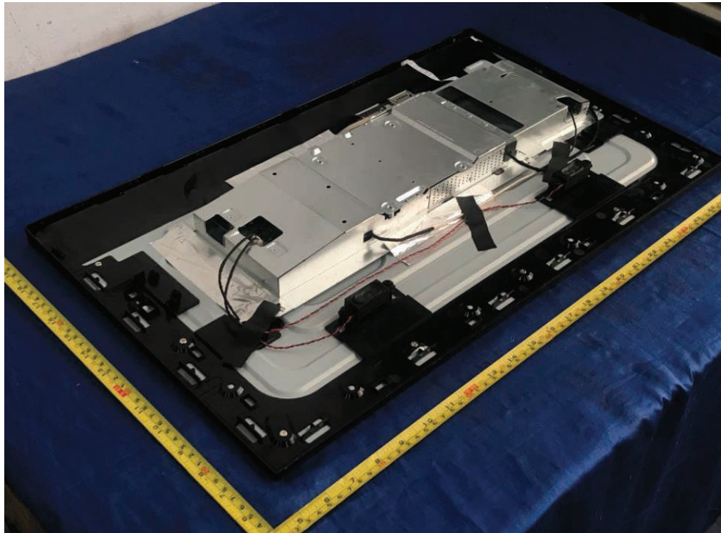
Figure 9. Metal enclosure type A
