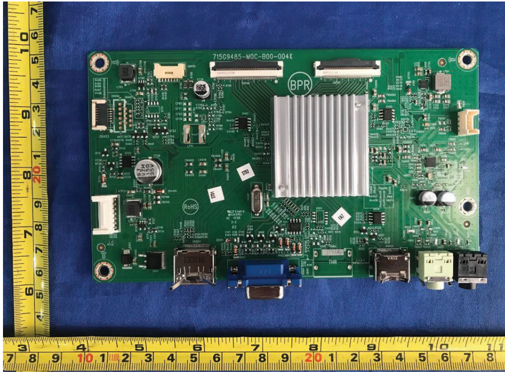
Figure 15. Main board 715G9485 type B
