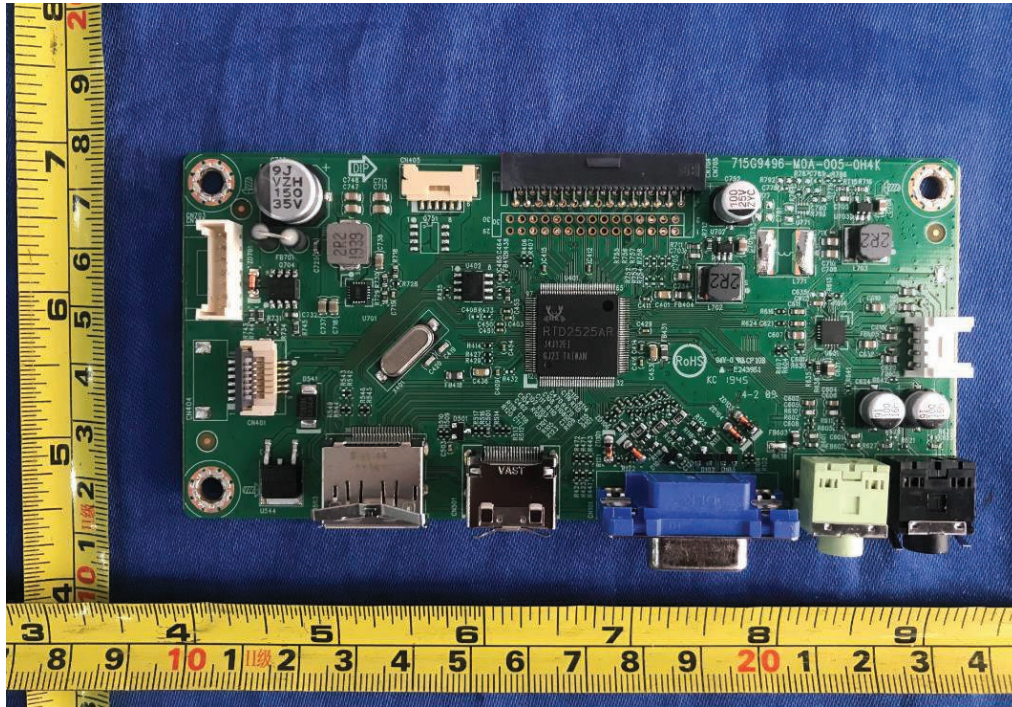
Figure 19. Main board 715G9496
