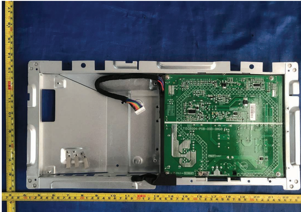
Figure 53. Internal view of metal enclosure
