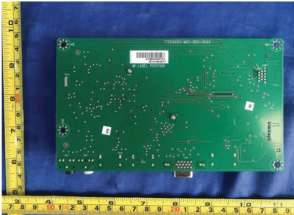
Figure 16. Main board 715G9485 type B
