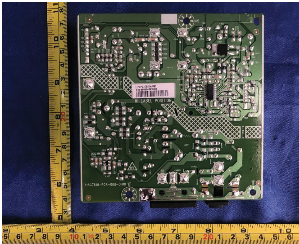
Figure 14. Power board 715G7610
