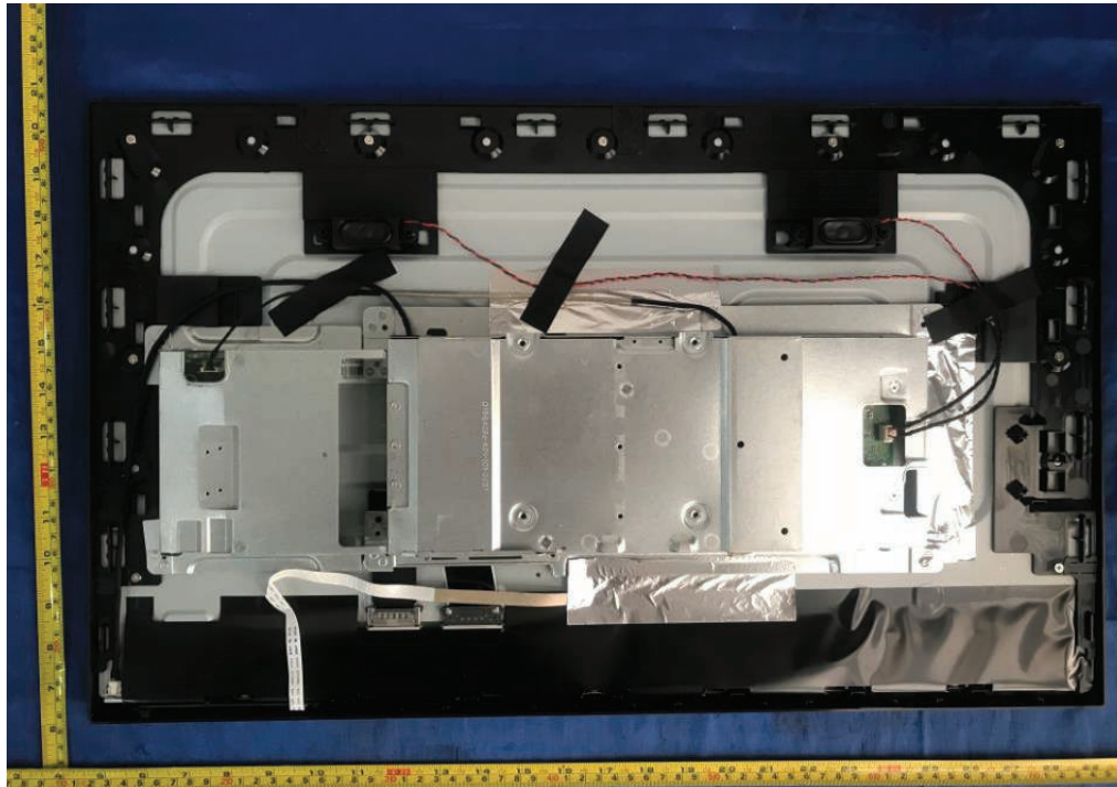
Figure 7. Metal enclosure type A
