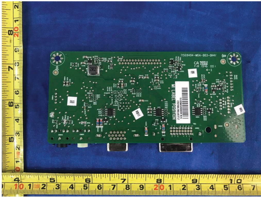
Figure 43. Main board 715G9494
