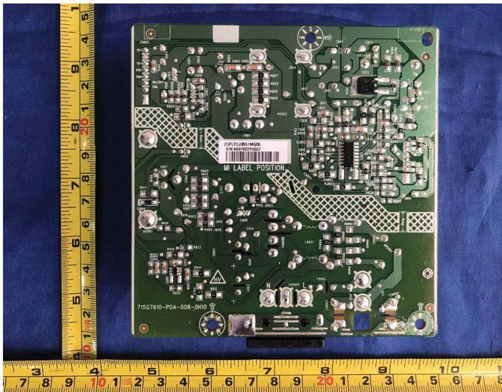
Figure 36. Power board 715G7610 (without AC switch)
