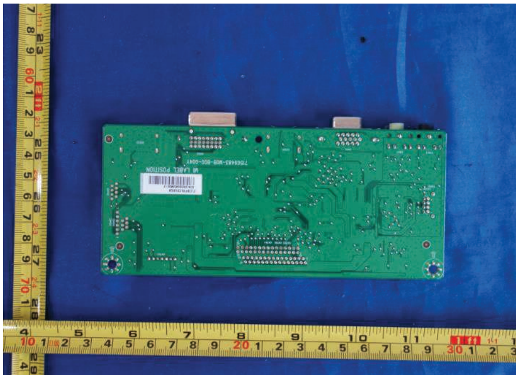
Figure 22. Main board 715G9483
