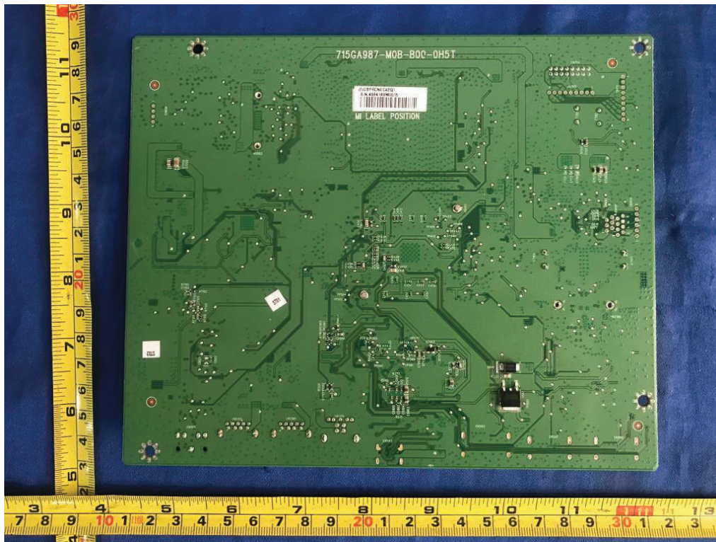
Figure 58. Main board 715GA987
