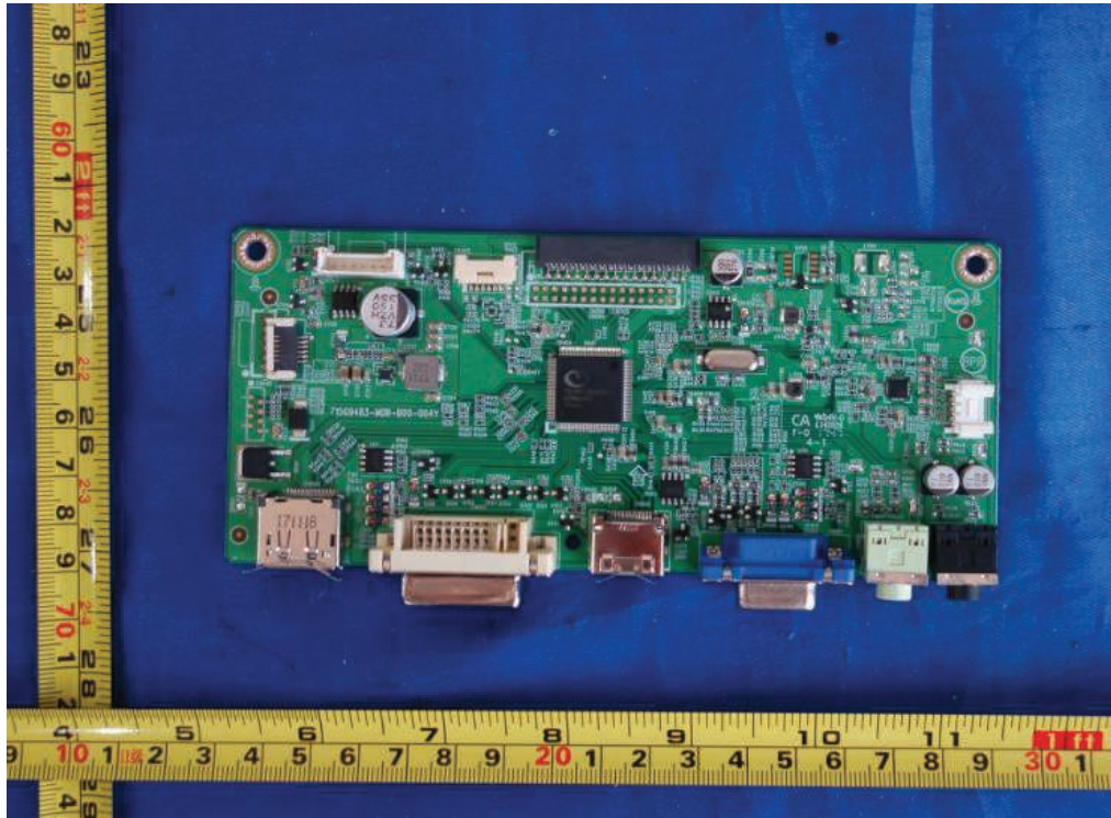
Figure 21. Main board 715G9483
