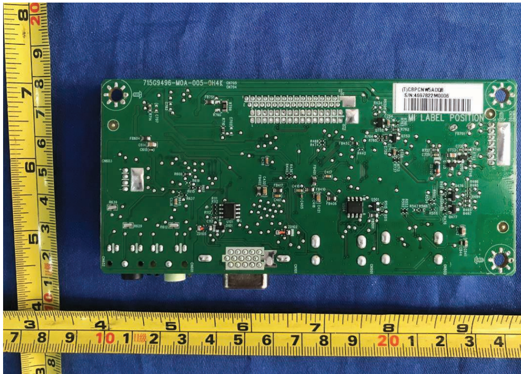
Figure 20. Main board 715G9496
