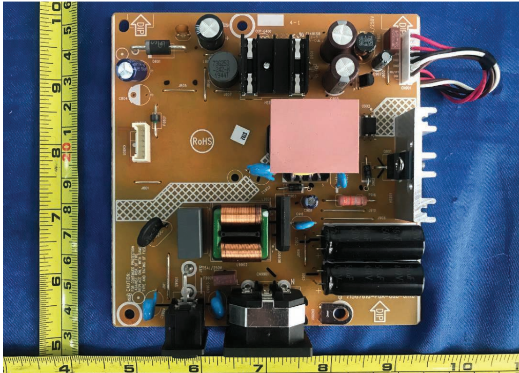
Figure 13. Power board 715G7610
