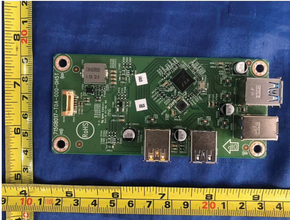
Figure 23. USB board 715GB017
