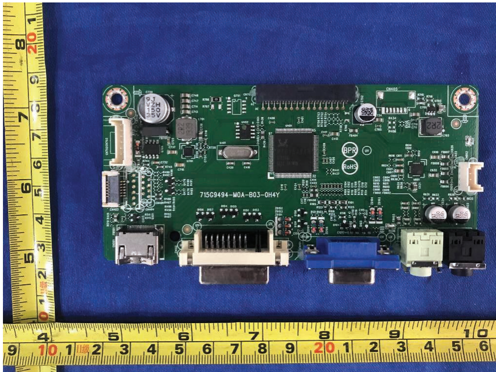
Figure 42. Main board 715G9494
