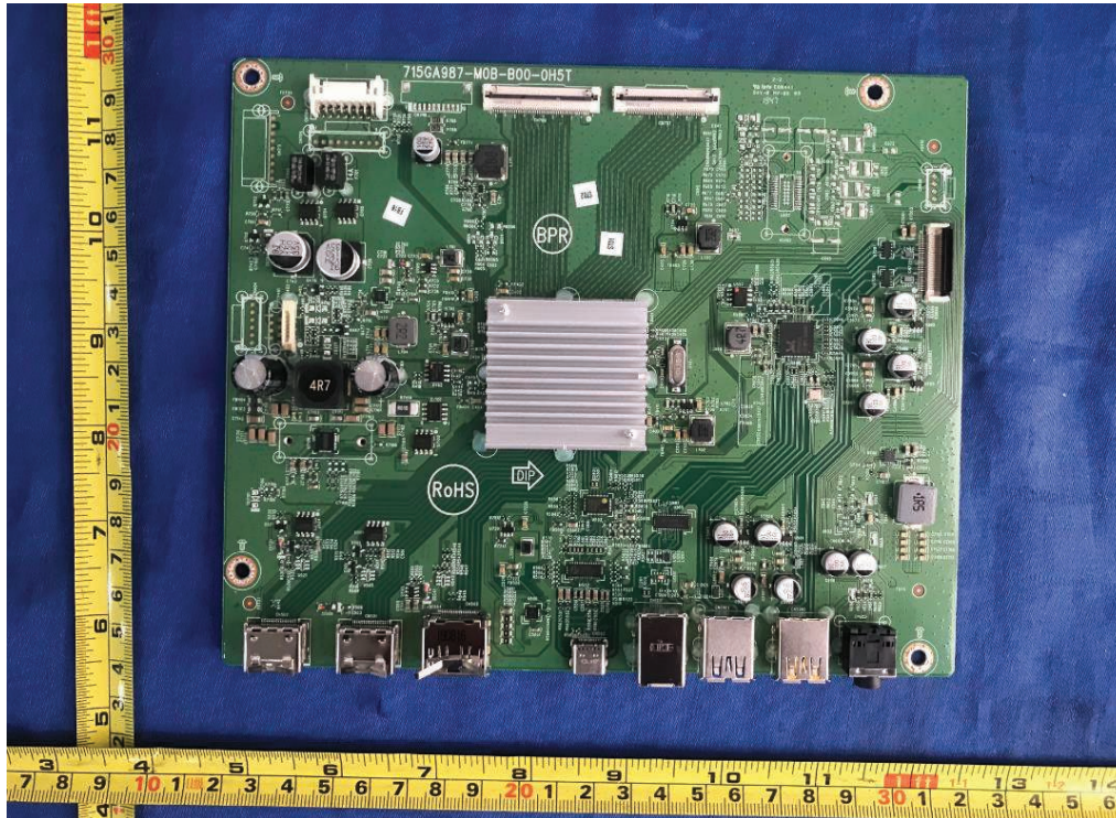
Figure 57. Main board 715GA987
