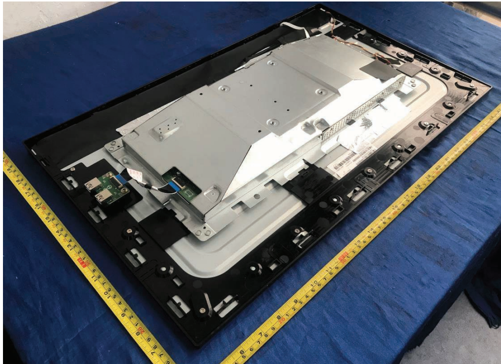
Figure 51. Metal enclosure type C
