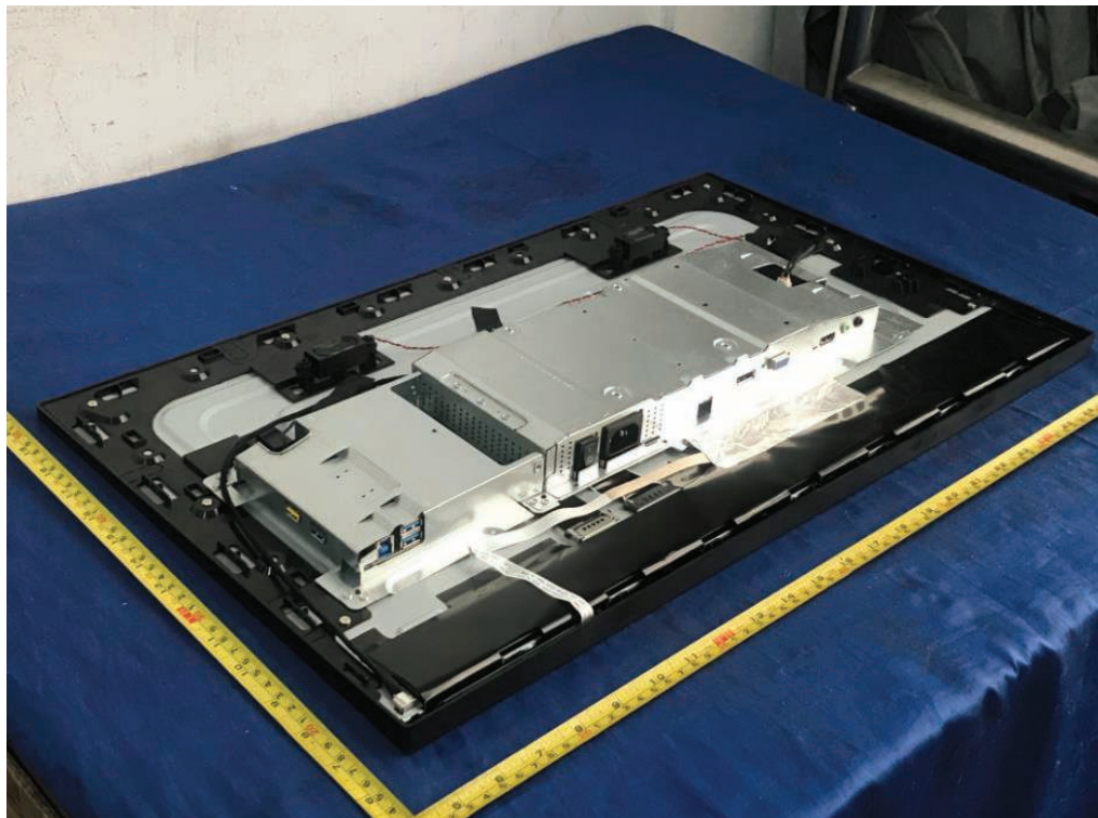
Figure 8. Metal enclosure type A
