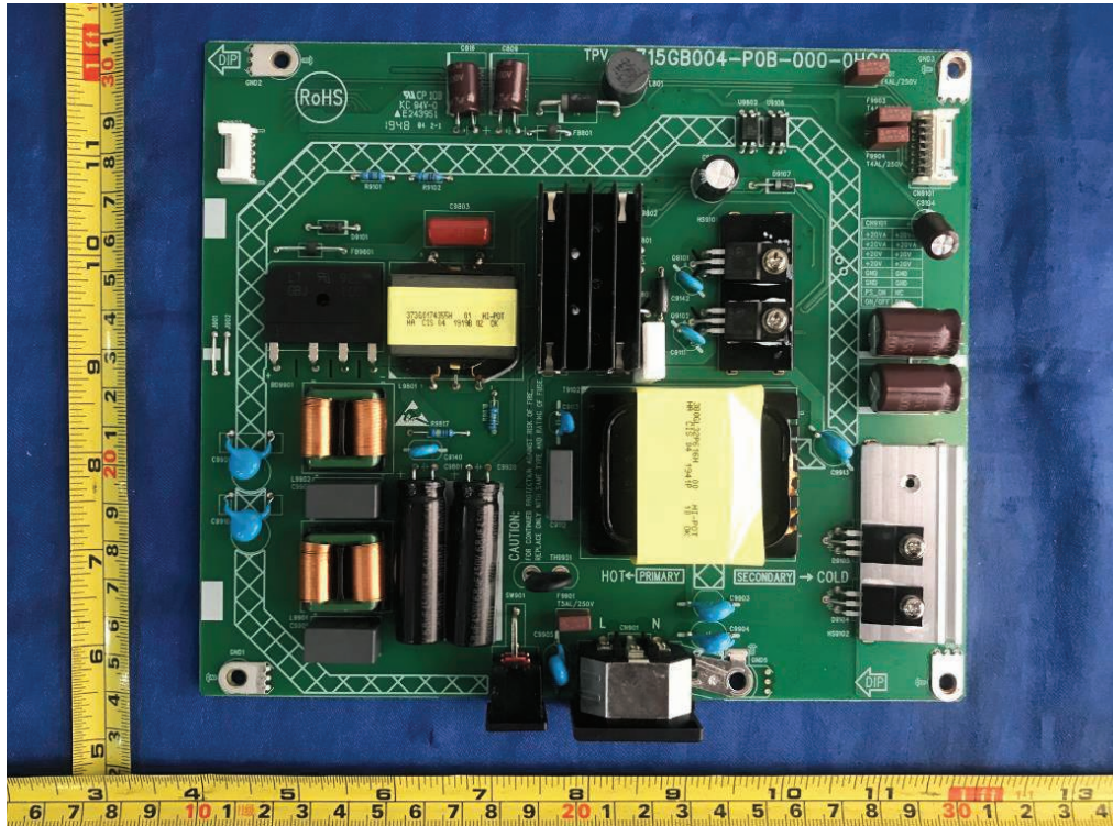
Figure 55. Power board 715GB004
