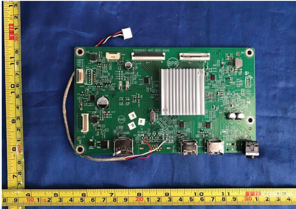
Figure 17. Main board 715G9485 type A
