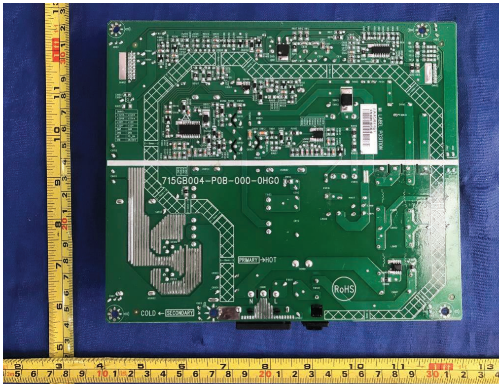
Figure 56. Power board 715GB004
