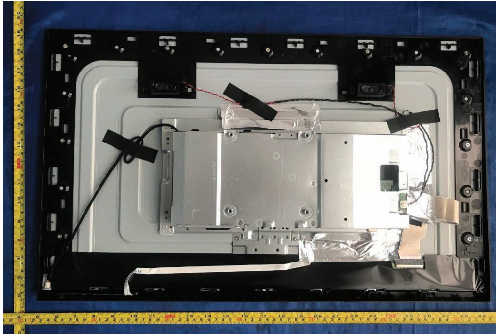
Figure 29. Metal enclosure type B
