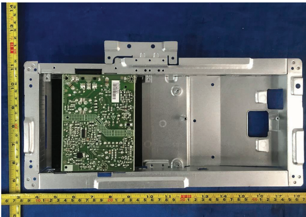
Figure 38. Internal view of metal enclosure
