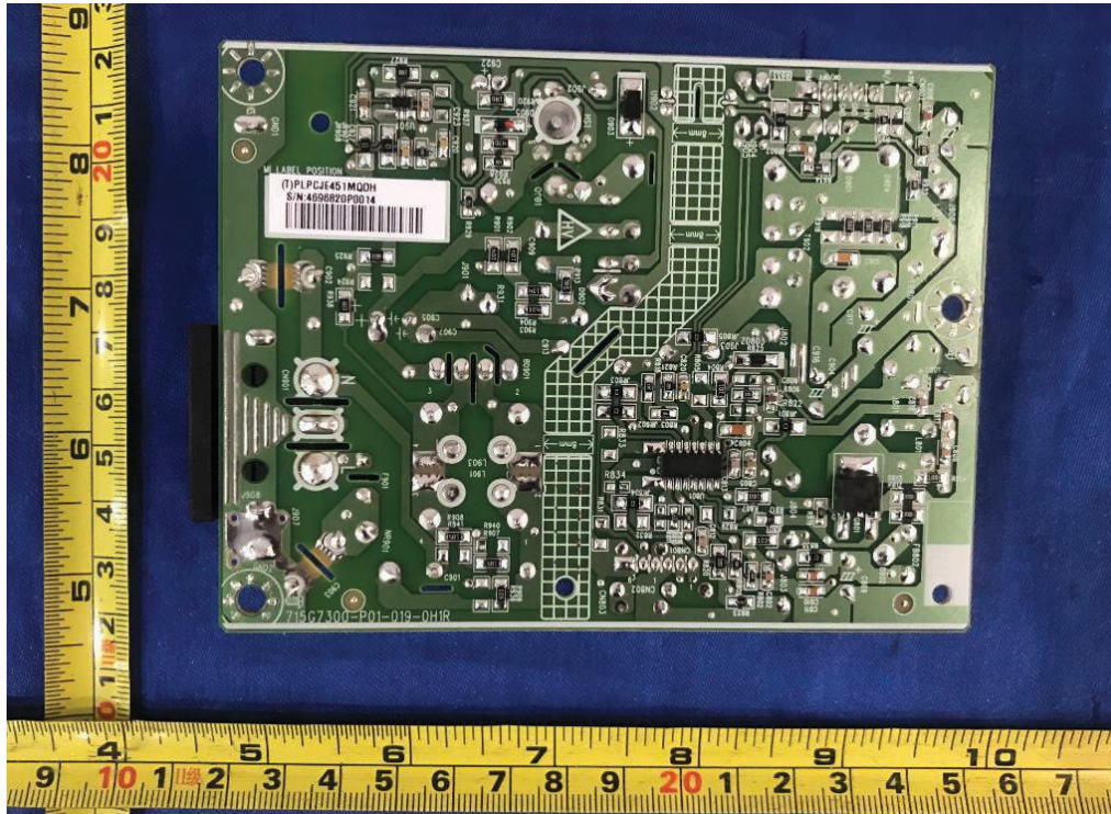
Figure 41. Power board 715G7300
