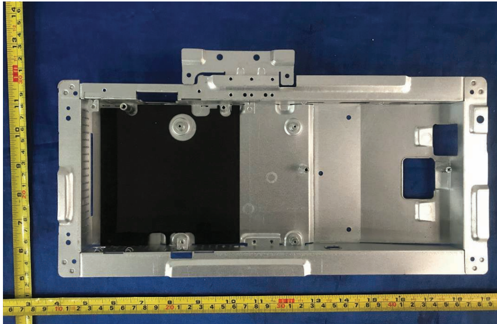
Figure 39. Internal view of metal enclosure
