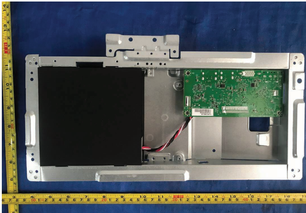
Figure 32. Internal view of metal enclosure type B
