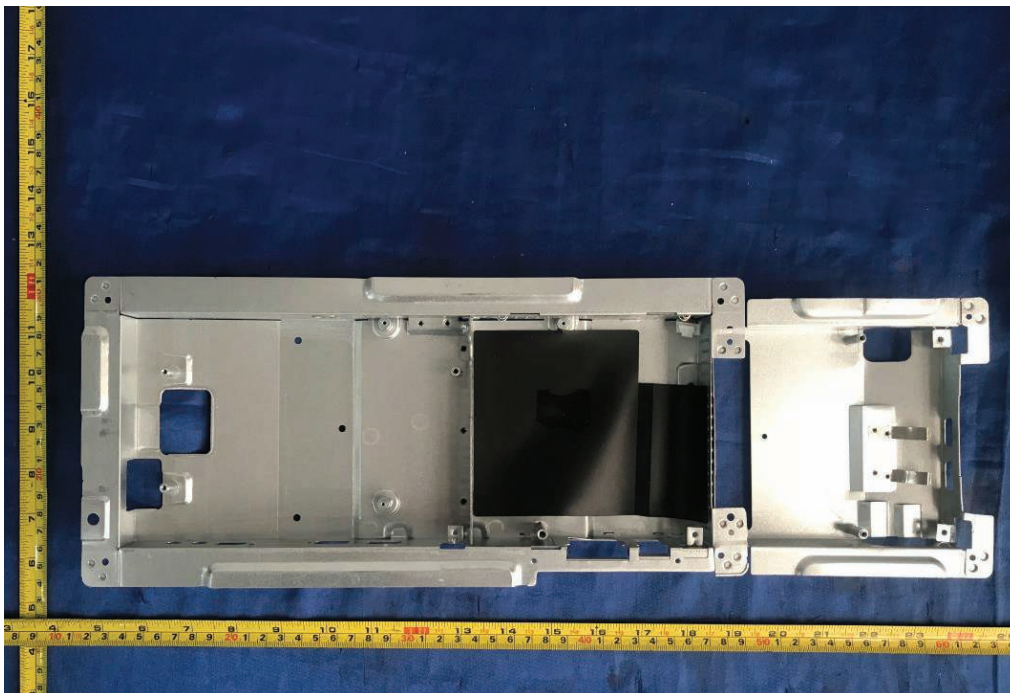
Figure 12. Internal view of metal enclosure type A
