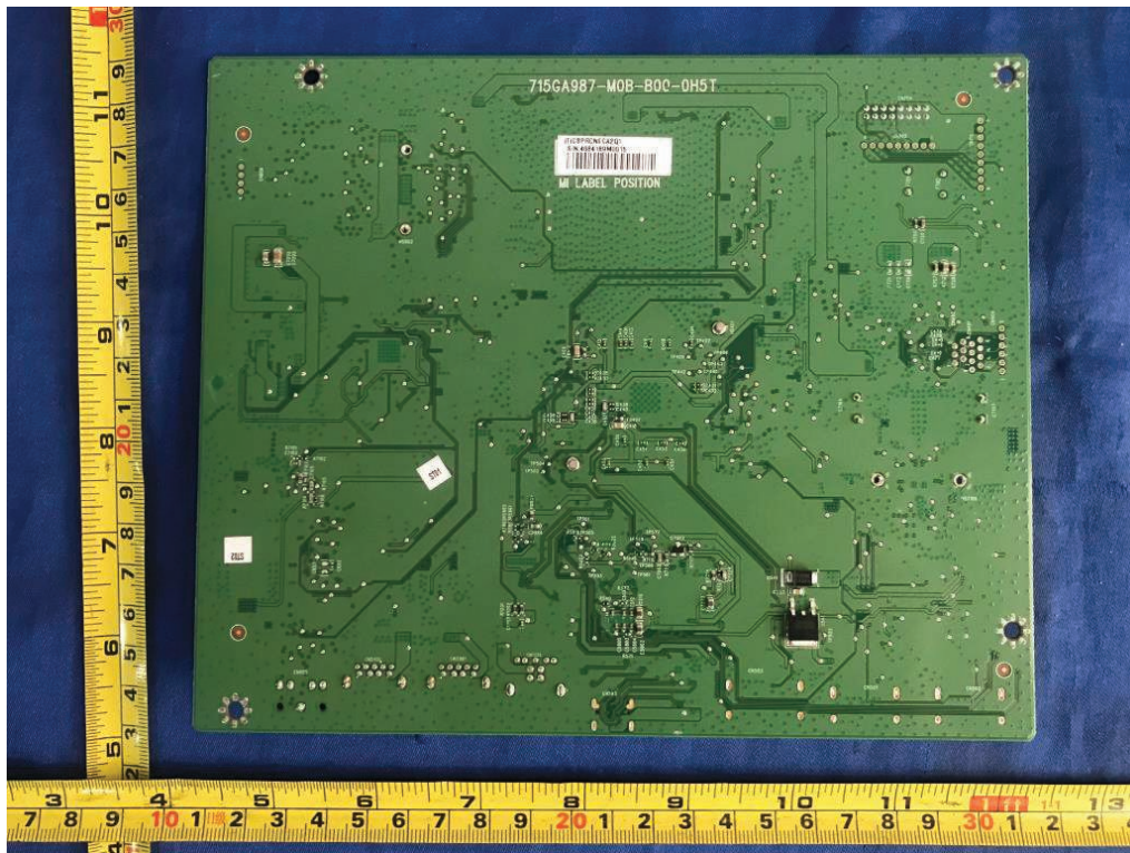
Figure 58. Main board 715GA987
