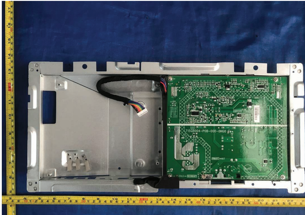
Figure 53. Internal view of metal enclosure
