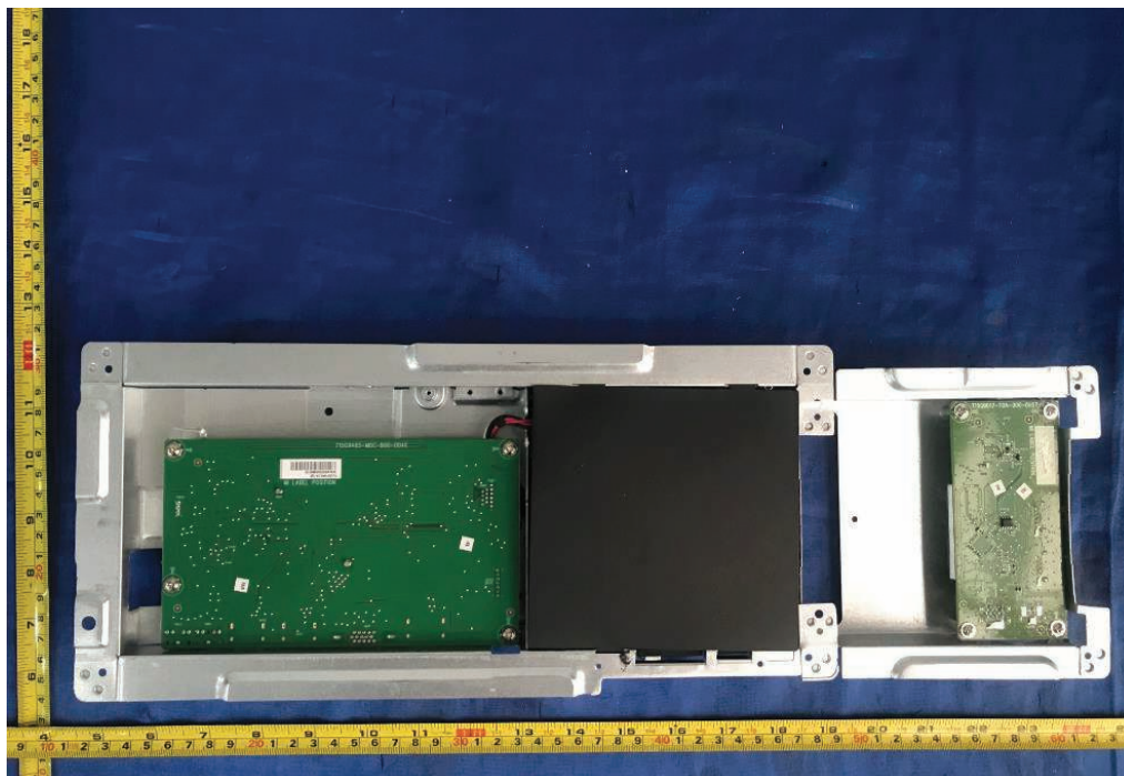
Figure 10. Internal view of metal enclosure type A
