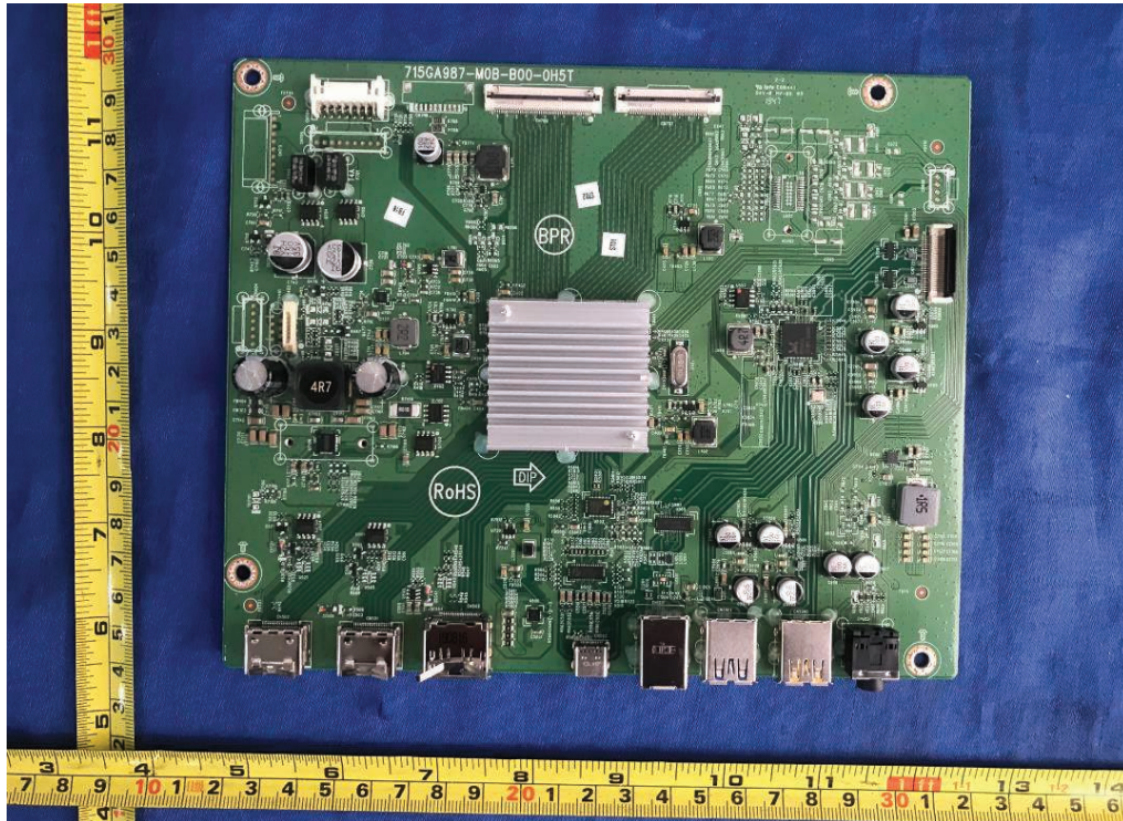
Figure 57. Main board 715GA987
