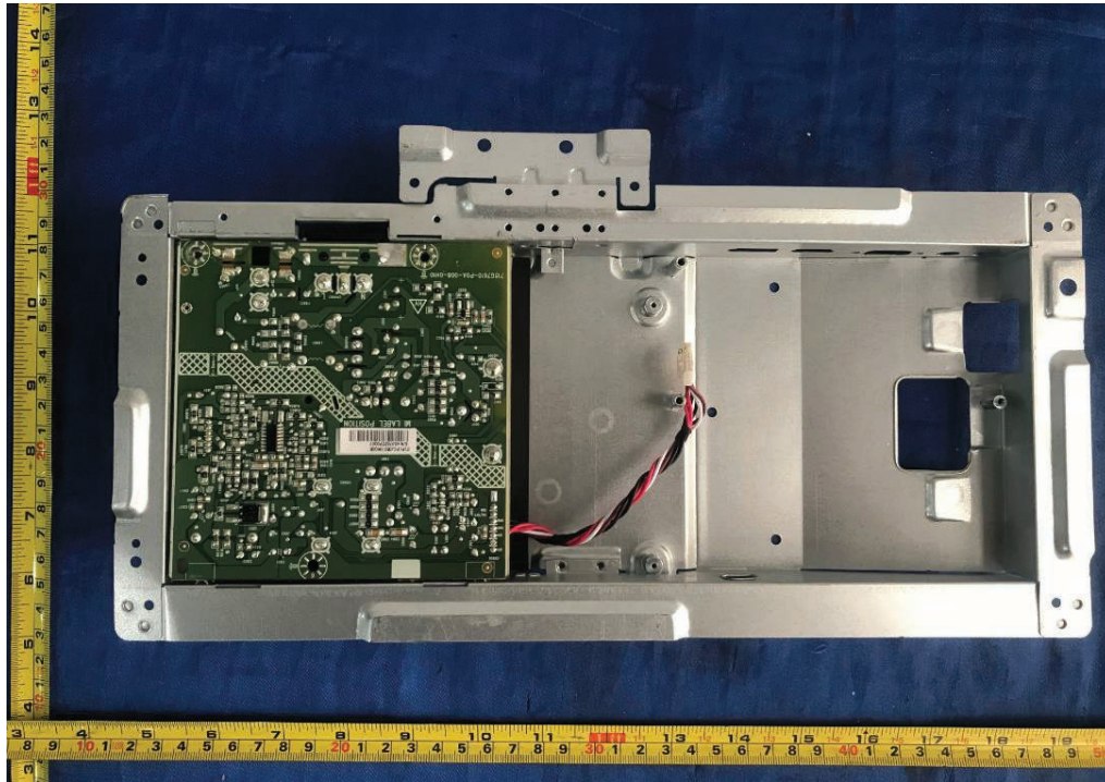
Figure 33. Internal view of metal enclosure type B
