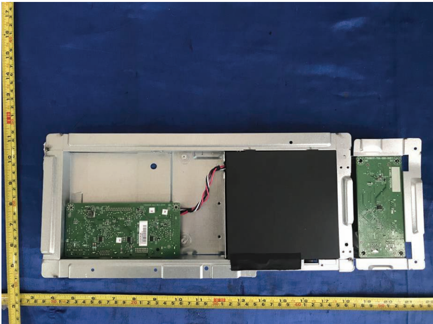
Figure 12. Internal view
