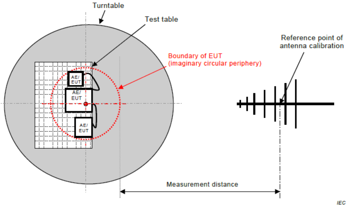
Figure C.1 – Measurement distance
