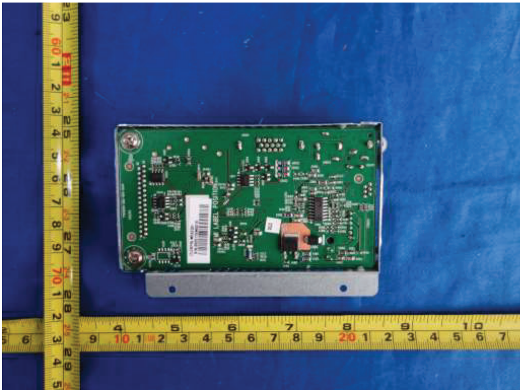
Figure 8. Internal view
