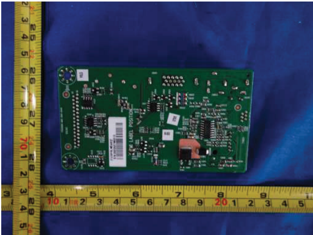
Figure 10. Main board 715G9284
