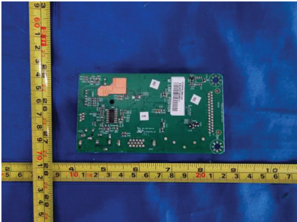
Figure 12. Main board 715G9353
