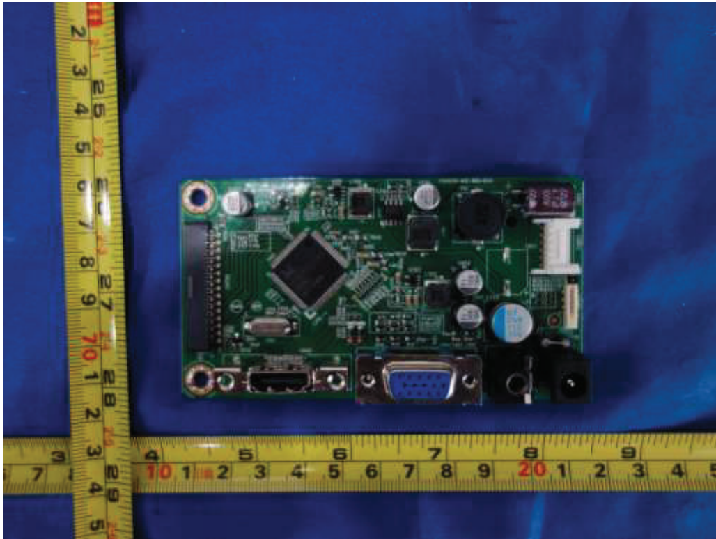
Figure 9. Main board 715G9284
