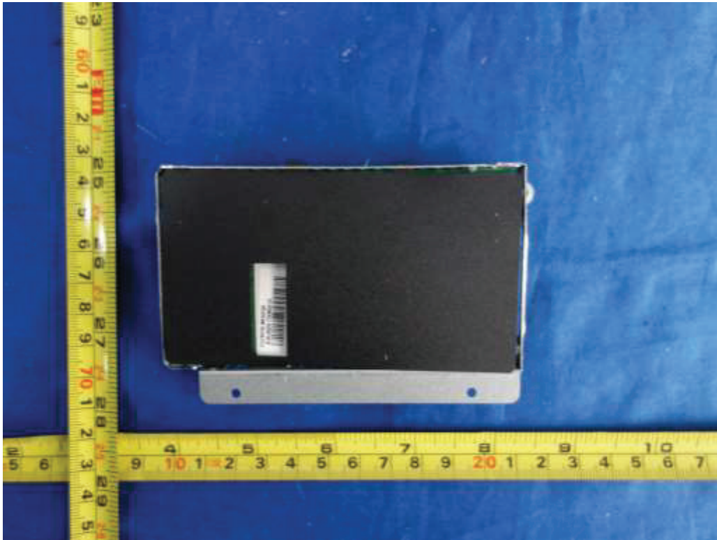
Figure 7. Internal view
