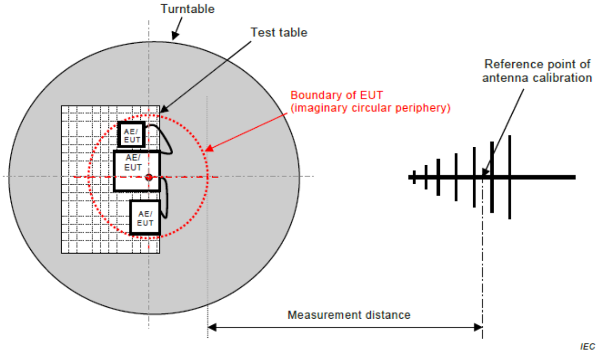
Figure C.1 – Measurement distance
