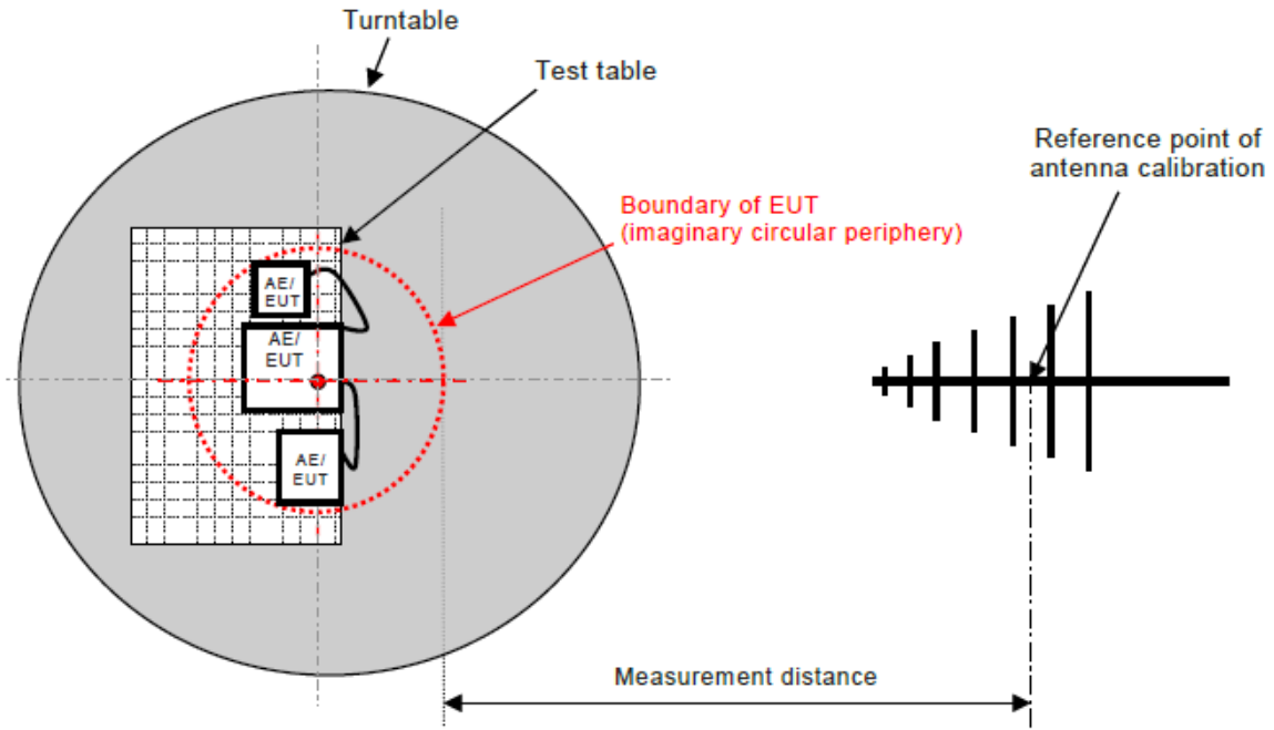
Figure C.1 – Measurement distance
