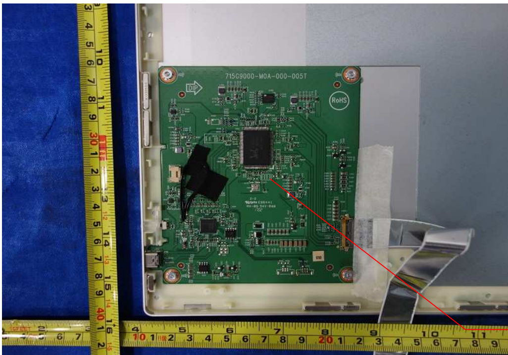
Photo 2 - Main Board (TPV/ 715G9000)
