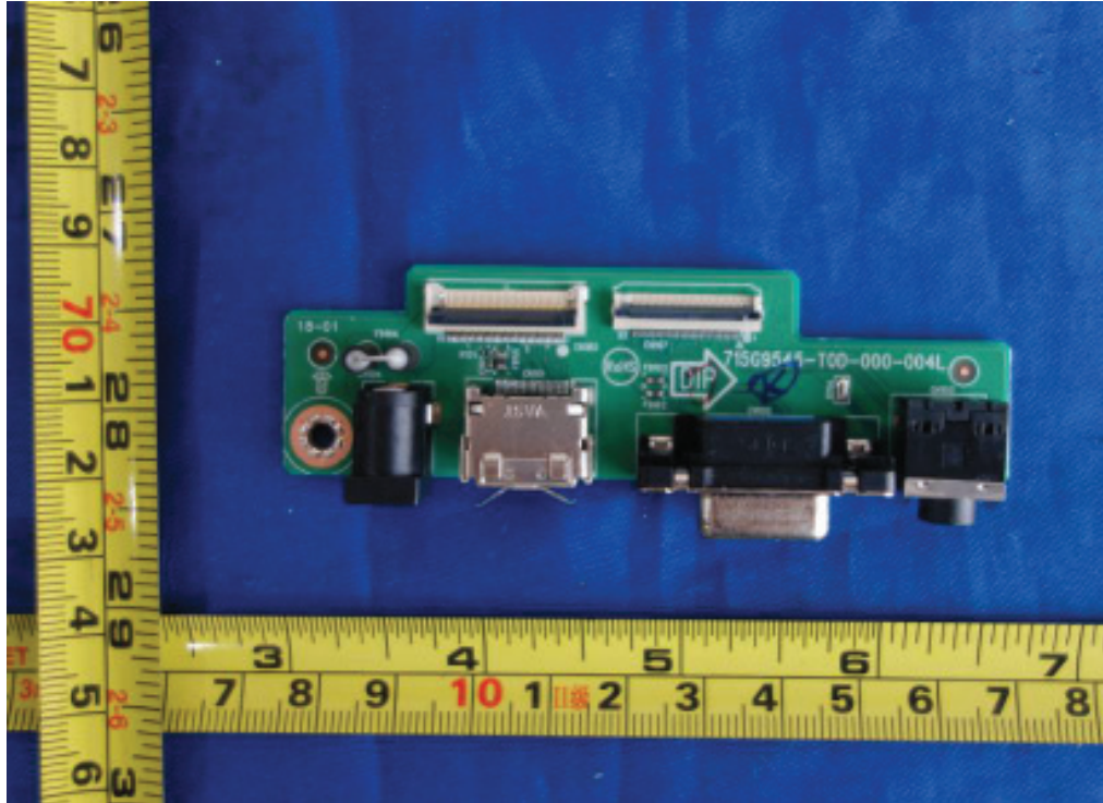
Figure 11. Connection board 715G9545
