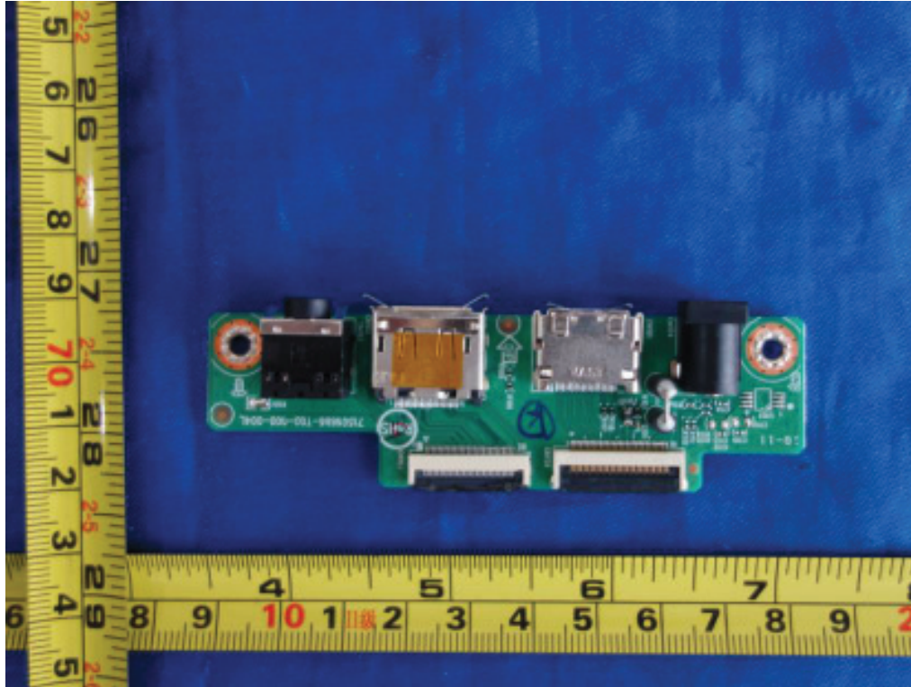
Figure 13. Connection board 715G9686
