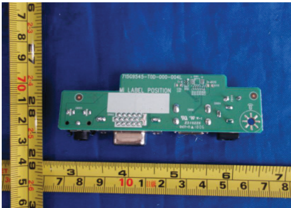
Figure 12. Connection board 715G9545
