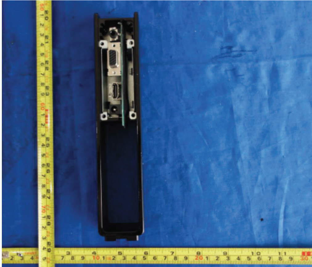
Figure 5. Internal view of base stand
