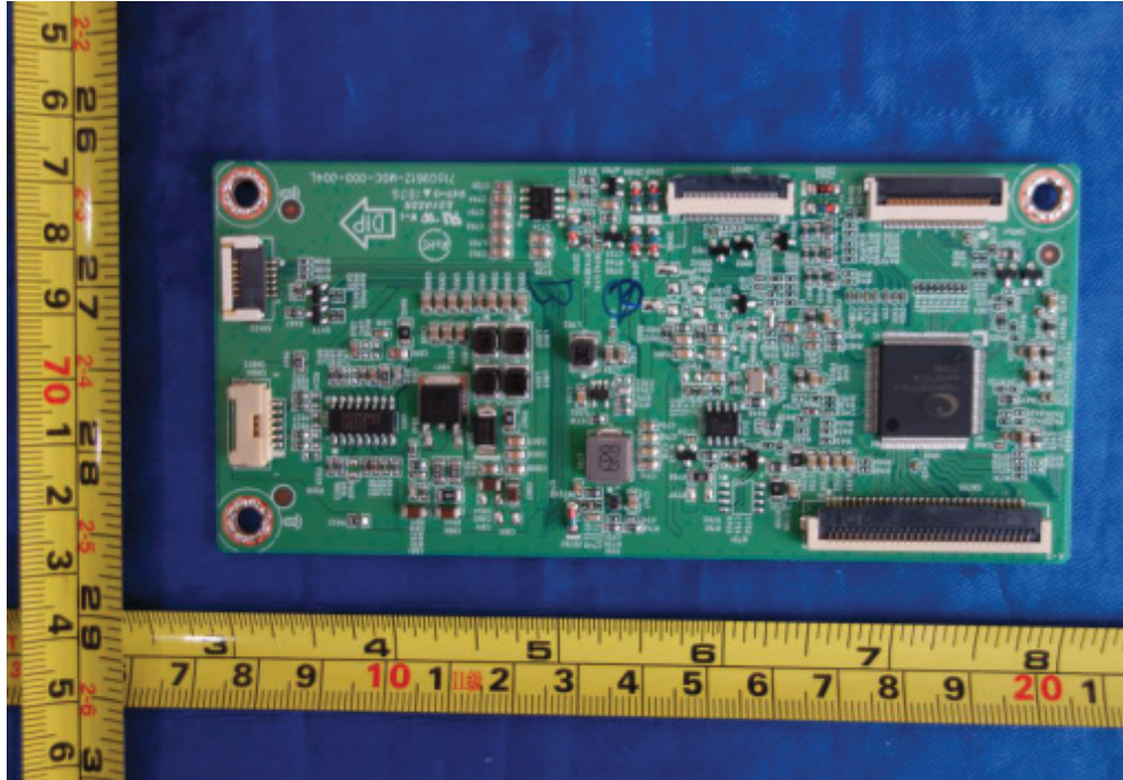
Figure 7. Main board 715G9612
