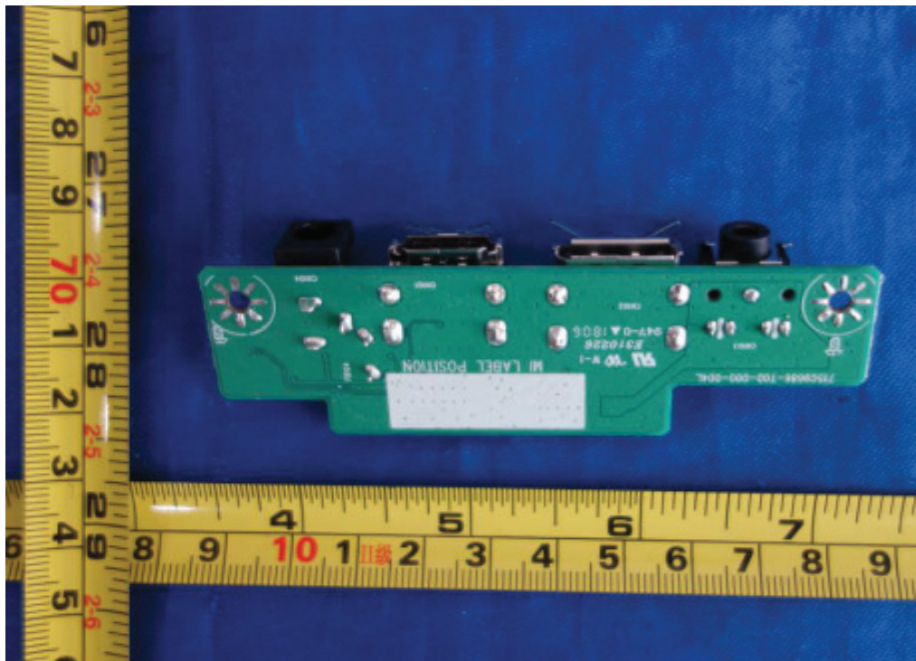
Figure 14. Connection board 715G9686
