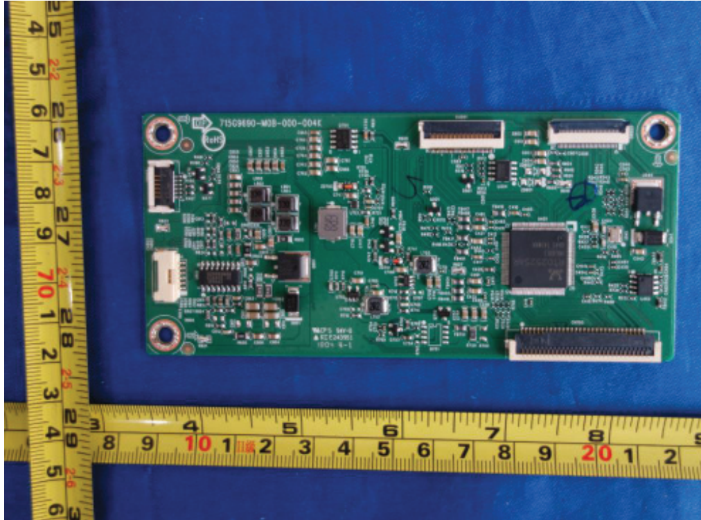
Figure 9. Main board 715G9690
