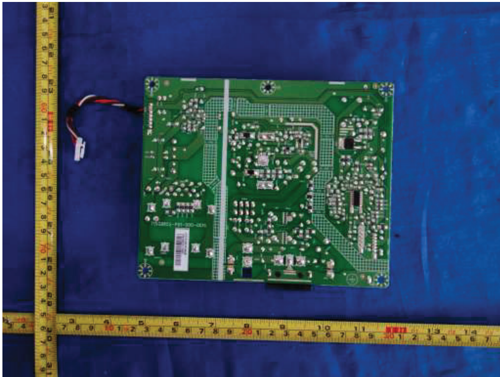
Figure 17. Main board 715G9250
