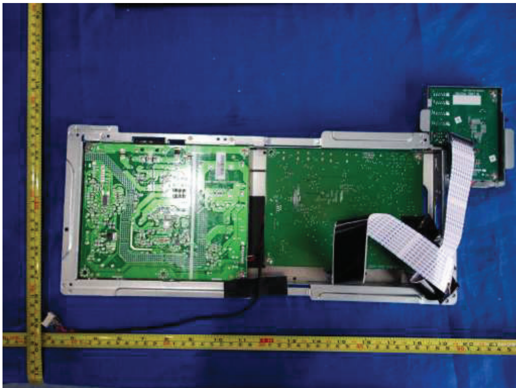
Figure 12. Internal view of metal enclosure with main board 715G9250
