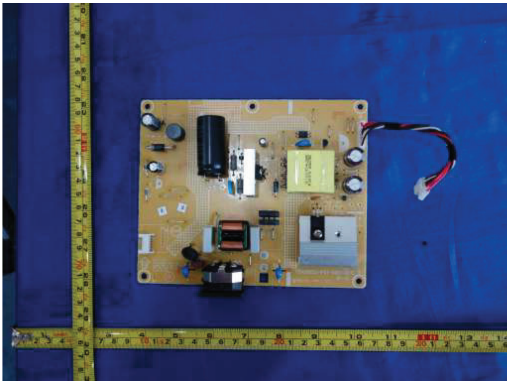
Figure 14. Power board 715G8852
