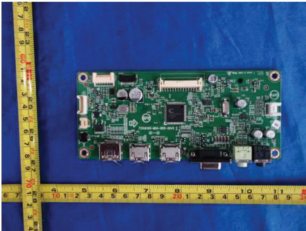
Figure 18. Main board 715G9260
