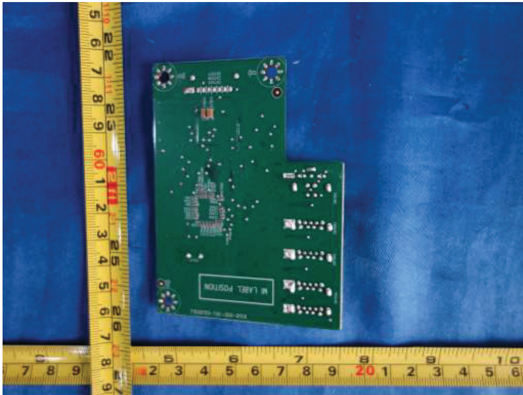
Figure 21. USB board 715G8765
