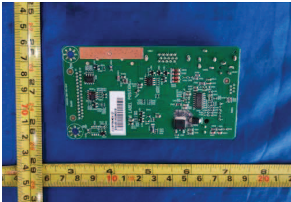
Figure 8. Main board 715G9284
