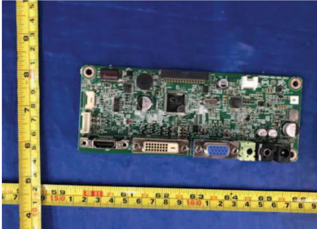
Figure 9. Main board 715G9620
