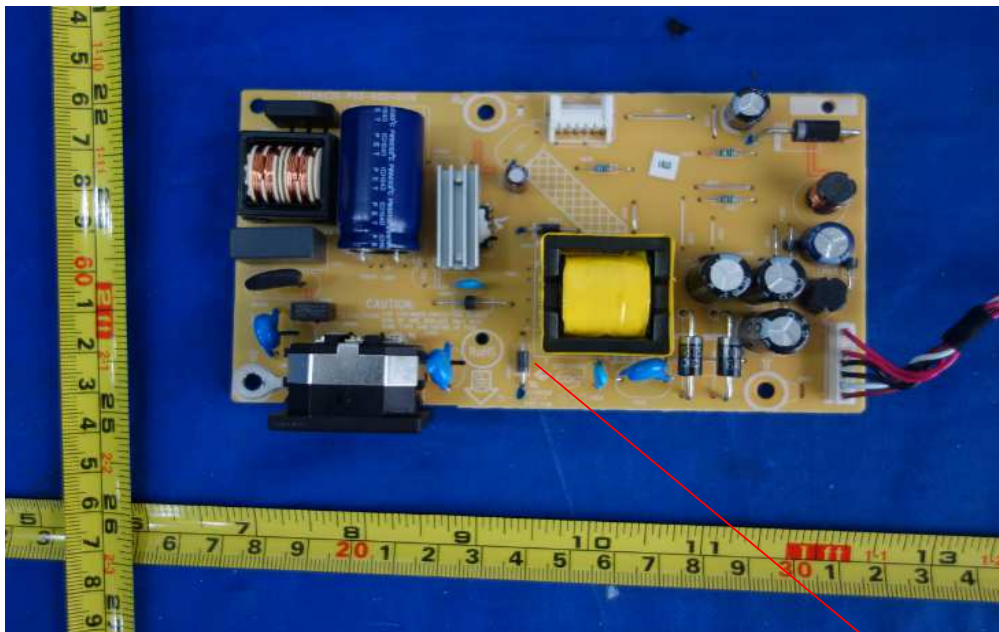
Photo 4 - Power Board
