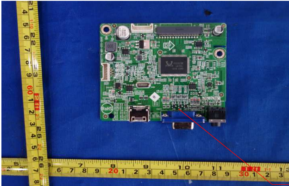
Photo 3 - Main Board
