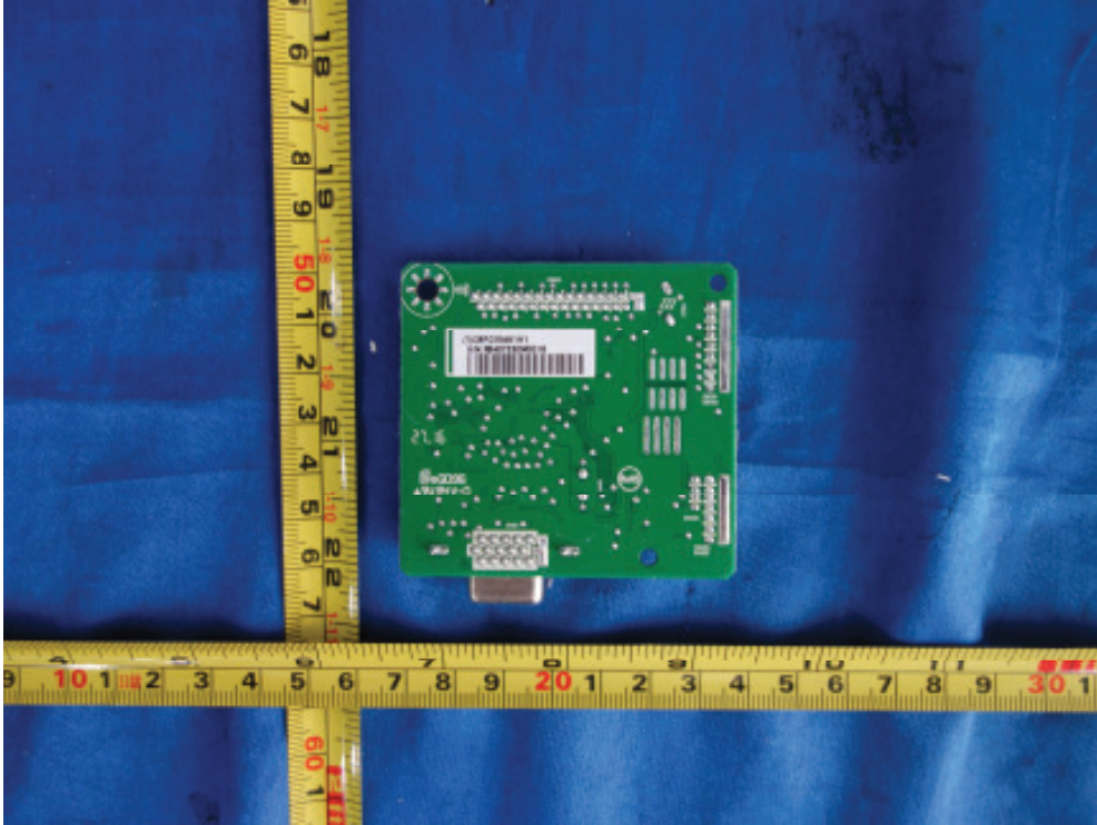
Figure 33. Main board 715G6851 type B
