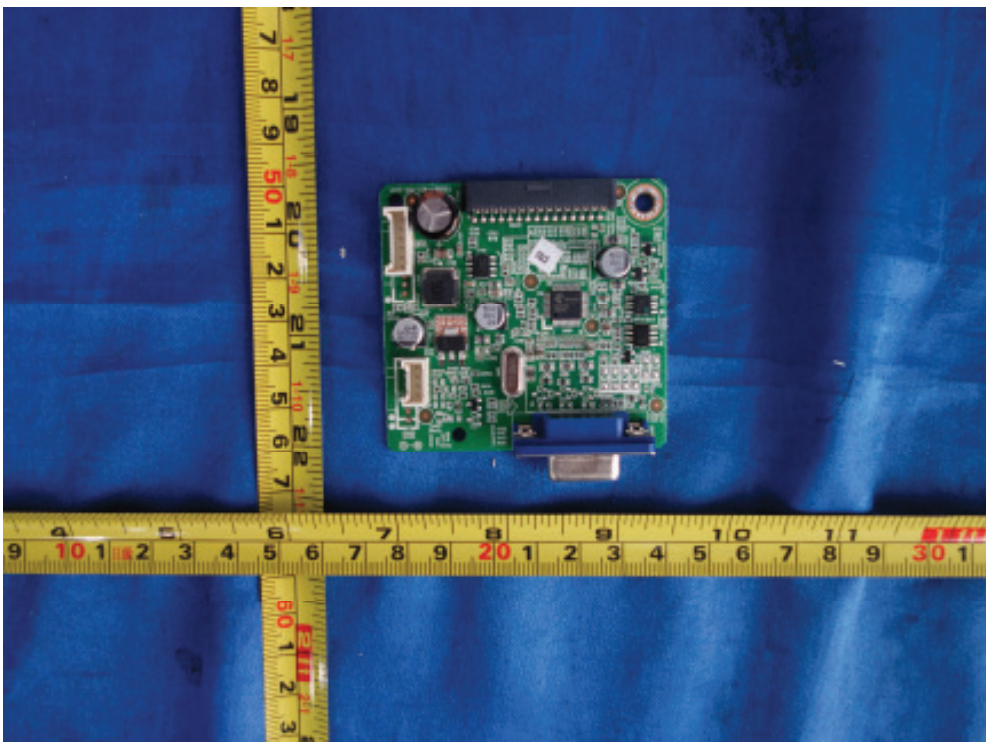
Figure 32. Main board 715G6851 type B
