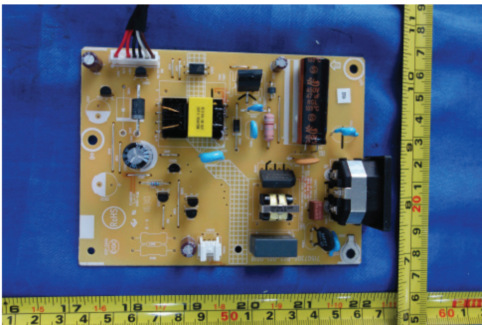
Figure 24. Power board 715G7300
