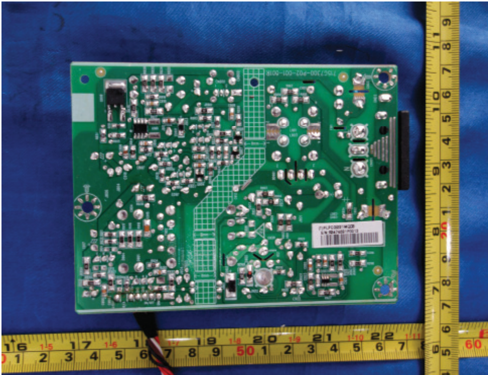
Figure 25. Power board 715G7300
