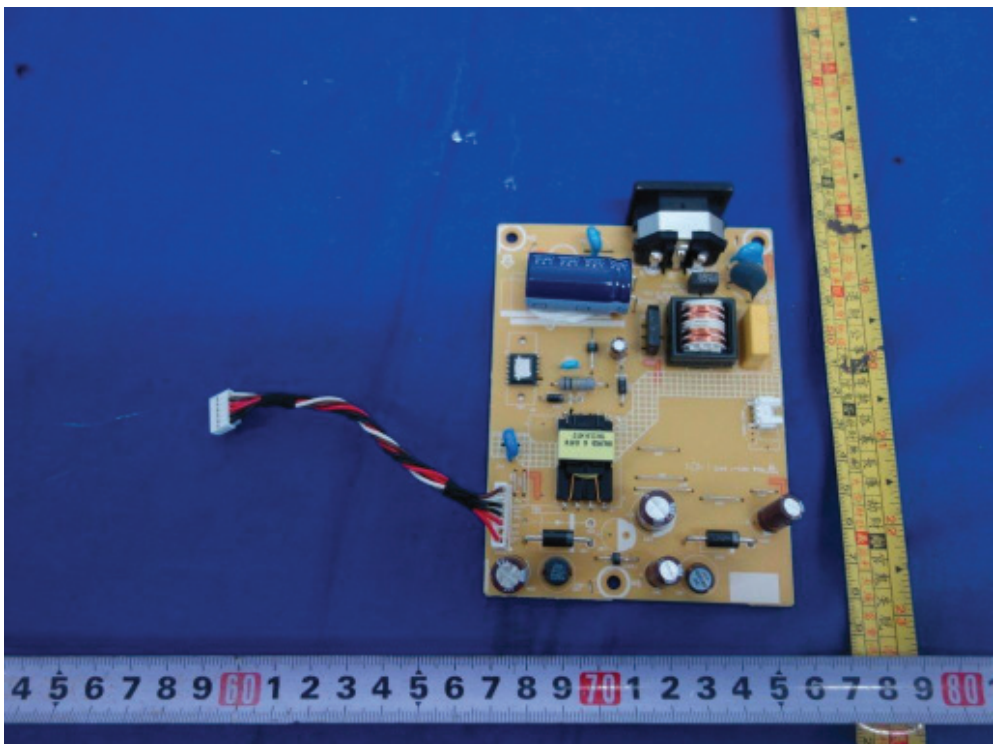
Figure 22. Power board 715G6503
