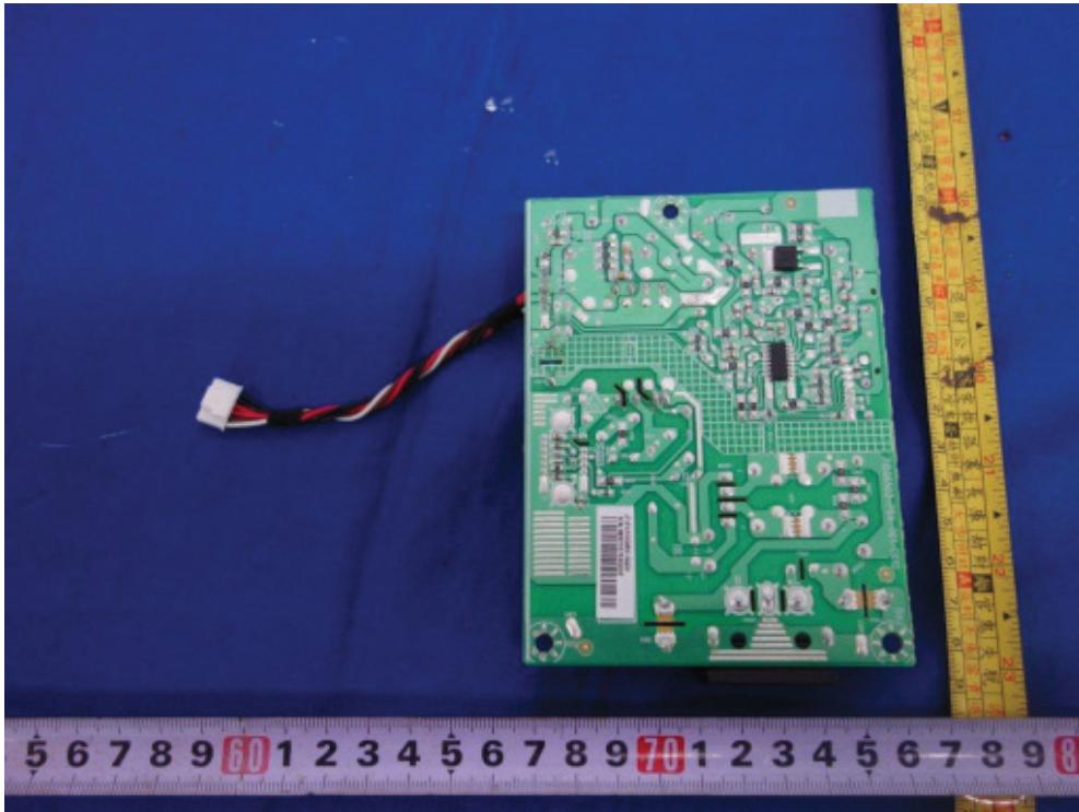
Figure 23. Power board 715G6503
