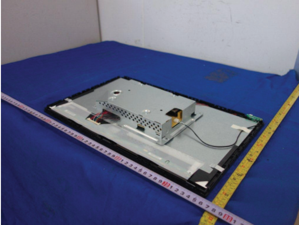
Figure 15. Metal enclosure type B
