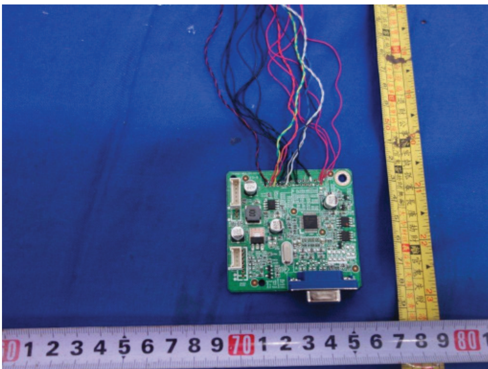
Figure 30. Main board 715G6851 type A
