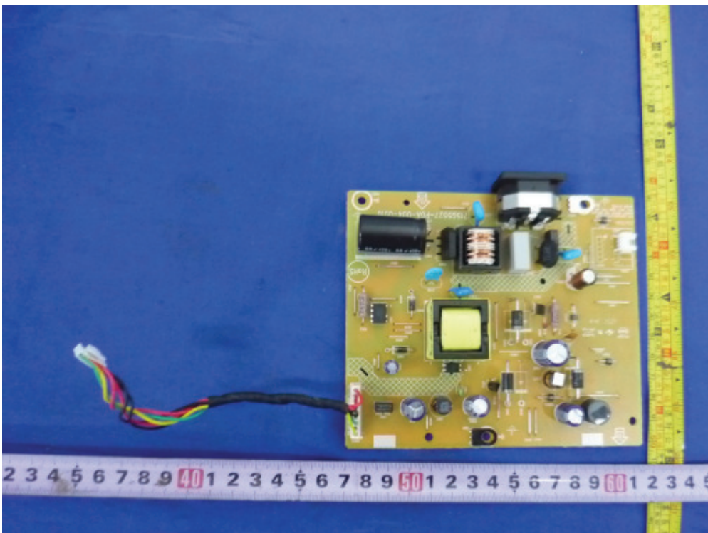
Figure 20. Power board 715G5527
